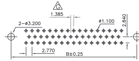
P.C. Board Layout (50 Positions)
