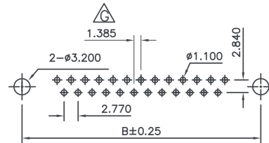
P.C. Board Layout (9,15,25,37 Positions)
